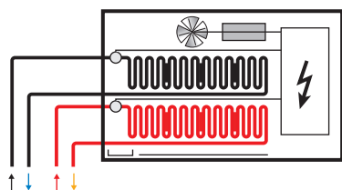
fan coil a 4 tubi
