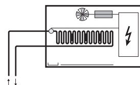
fan coil a 2 tubi
