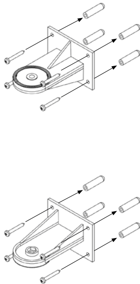
FISSAGGIO STAFFA A MURO FIXING THE BRACKET TO THE WALL
